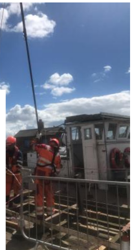
Pictured below right: Reach and Rescue's Inspection Camera is used to inspect underneath the hulls of sea vessels, saving considerable time and effort.
